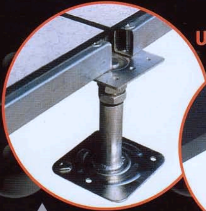
▲ Bolted Stringer
